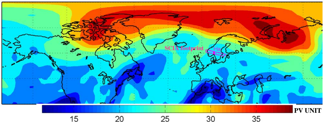
Fig. 3: Potential Vorticity (PV) map at 475 K for 16/04/2004.
