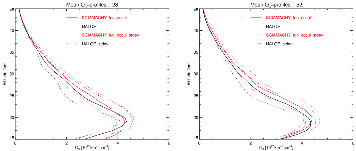
Figure 7. SCIAMACHY-HALOE mean ozone profiles for 2003 (28 coincidences) and 2004 (52 coincidences). Red is the SCIAMACHY result and black the HALOE result. The dotted lines are the standard deviations of the mean profiles.
