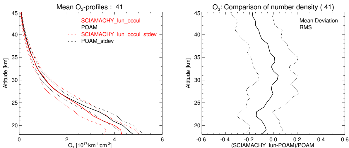
Figure 10. Left: SCIAMACHY-POAM mean ozone profiles for 2003 (41 coincidences). Right: the mean relative deviations (solid line) and the standard deviations of the relative deviations (dotted line) of the 41 SCIA-POAM III co-located observations.
