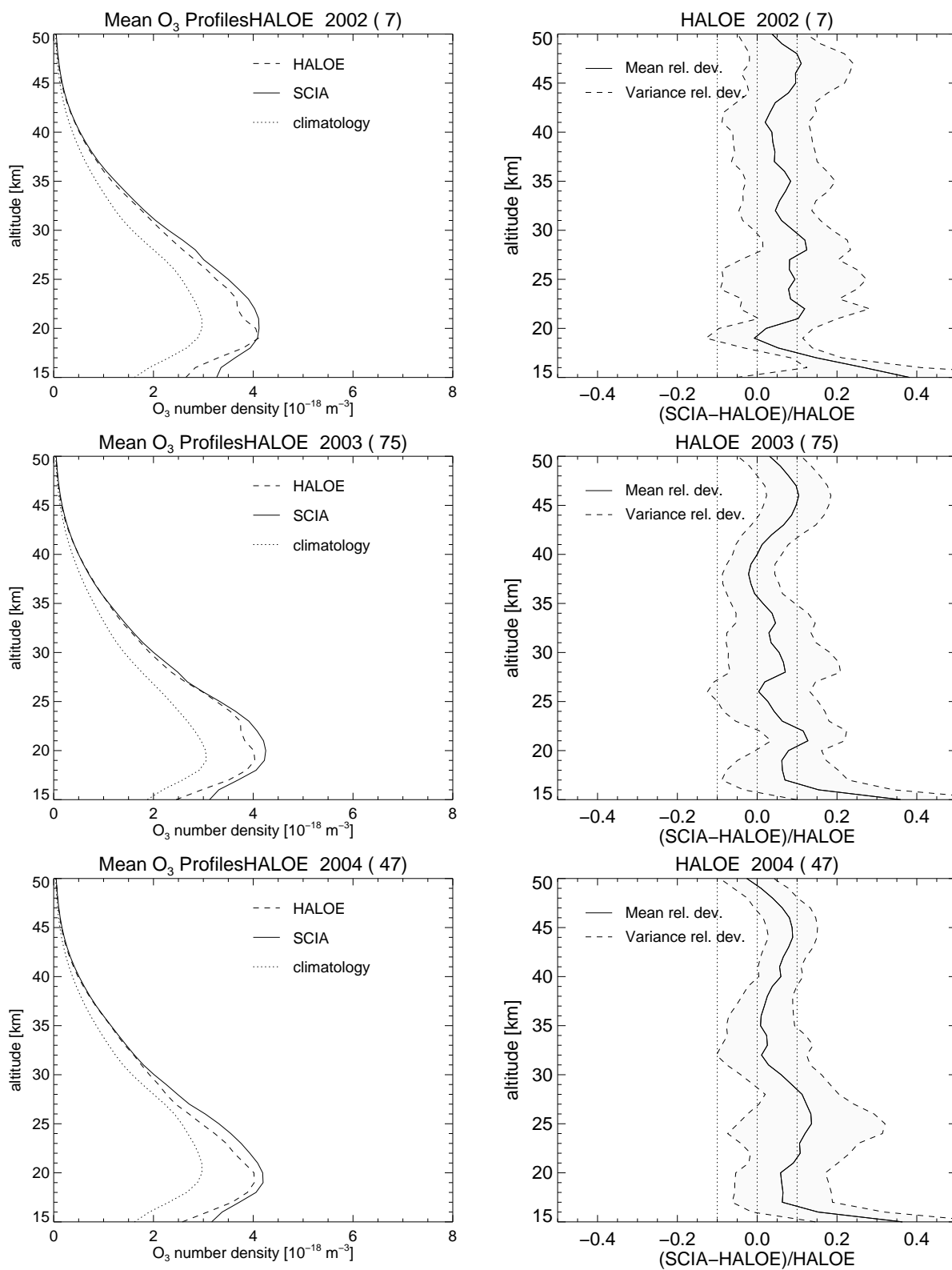
Figure 3. Validation results of ozone profiles from SCIAMACHY solar occultation with HALOE. Left column shows the mean profiles of the dataset (climatology is the a-priori profile used in the SCIAMACHY retrieval). Right column shows the mean relative deviation and its variance. From top to down: 2002 with 7 co-locations, 2003 with 75 co-location and 2004 with 47 co-locations.
