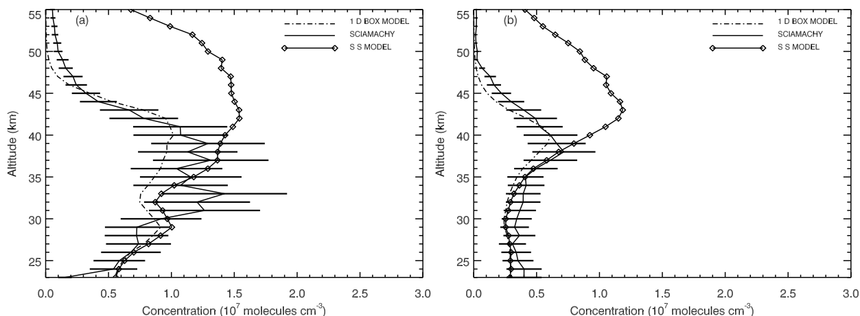
Figure 14. \text{NO}_3 profile retrieved compared with \text{NO}_3 profile calculated from the photochemical and steady state models. Solid line is the retrieval result, the dashed-dotted line is the photochemical model output and the solid line with diamond points is the steady state model results. (a) Example of \text{NO}_3 profiles for 14th March, 2003 (at SZA of 110^\circ ). (b) Example of \text{NO}_3 profile for 12th April, 2003 (at SZA of 115^\circ ).
