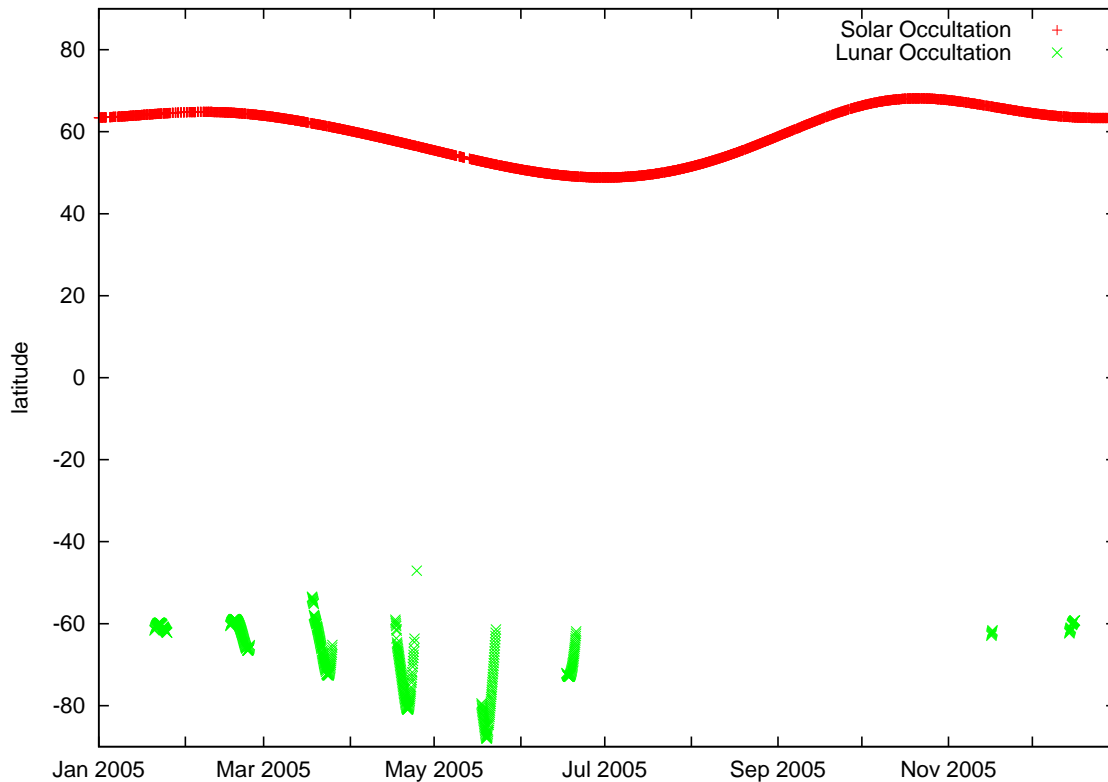
Figure 1. Latitudinal distribution of SCIAMACHY solar and lunar occultation measurements in 2005. Solar occultation measurements marked in red, lunar measurements in green.
