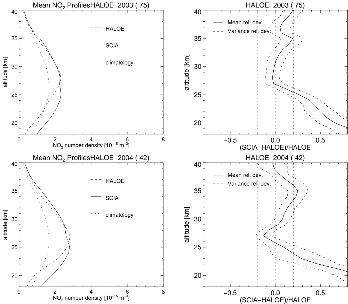
Figure 5. Validation results of \text{NO}_2 profiles from SCIAMACHY solar occultation with HALOE, like Figure 3. From top to down: 2003 with 75 co-location and 2004 with 42 co-locations.
