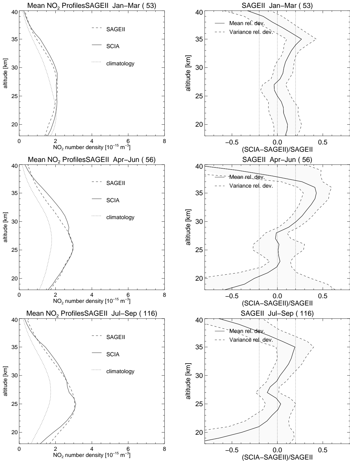
Figure 6. Validation results of NO 2 profiles from SCIAMACHY solar occultation with SAGEII, like Figure 4. From top to down: season January to March with 53 co-location, season April to June with 56 co-locations and season July to September with 116 co-locations.
