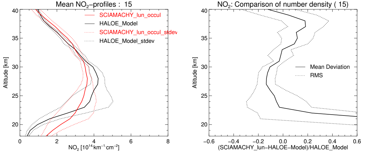
Figure 12. Left: mean \text{NO}_2 profile and corresponding standard deviation for 15 co-located events in 2003, SCIAMACHY version 2.2 in red and HALOE in black. Right: the mean relative deviation (solid line) and the standard deviation of the relative deviation (dotted line).
