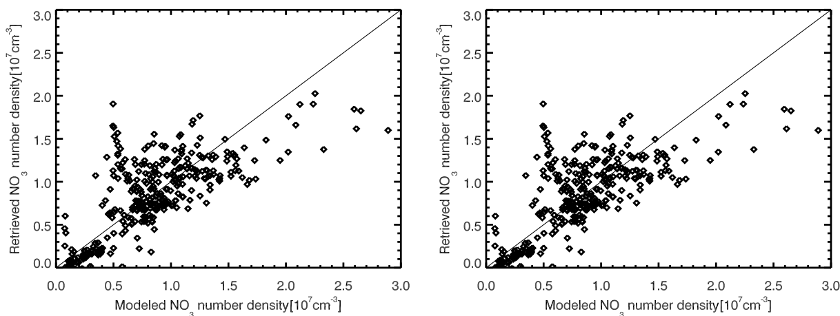
Figure 15. Retrieved \text{NO}_3 concentration from SCIAMACHY lunar occultation as a function of \text{NO}_3 calculated from the steady state model output. (a) The result for latitude band of (60-65^\circ \text{S}) , the correlation coefficient for this graph is 0.83. (b) The result for latitude band of (66-72^\circ \text{S}) the correlation coefficient for this graph is 0.98
