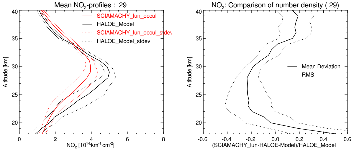
Figure 13. Left: mean NO 2 density profile and corresponding standard deviation for 29 co-located events in 2004, SCIAMACHY version 2.2 in red and HALOE in black. Right: the mean relative deviation (solid line) and the standard deviation of the relative deviation (dotted line).
