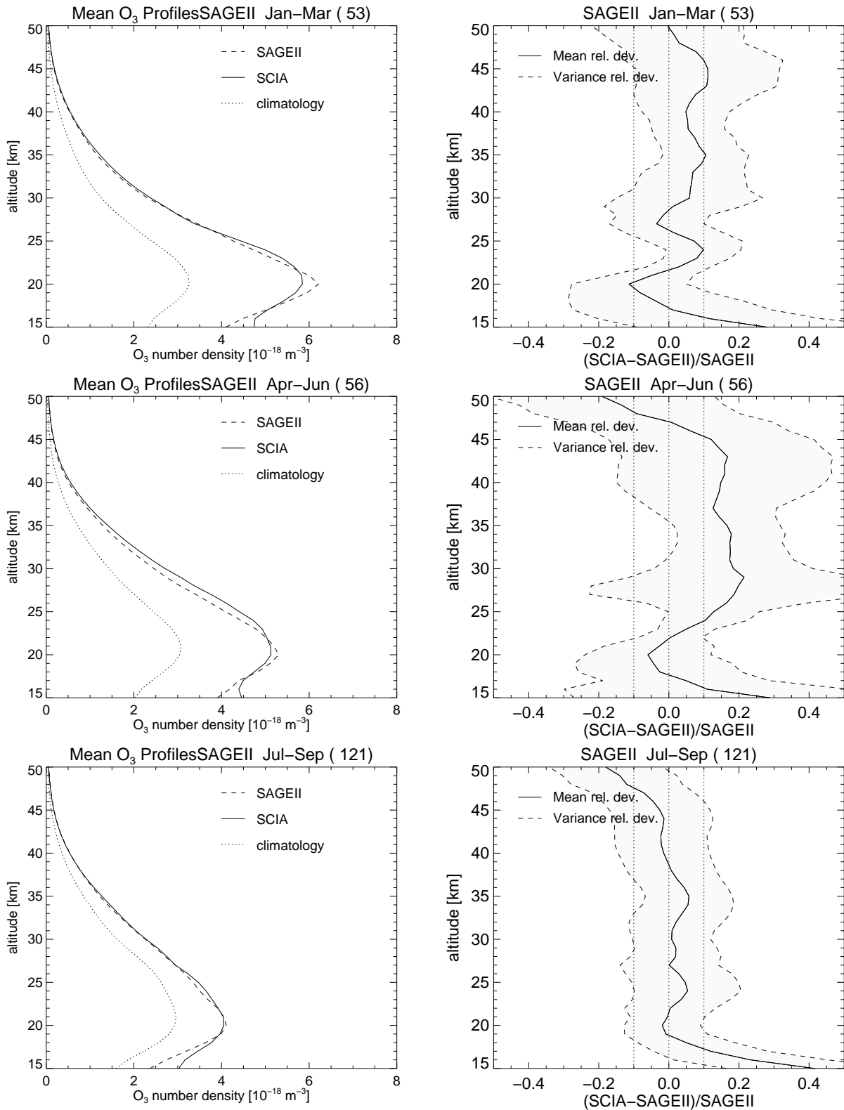
Figure 4. Validation results of ozone profiles from SCIAMACHY solar occultation with SAGE II, like Figure 3. From top to down: season January to March with 53 co-location, season April to June with 56 co-locations and season July to September with 121 co-locations.
