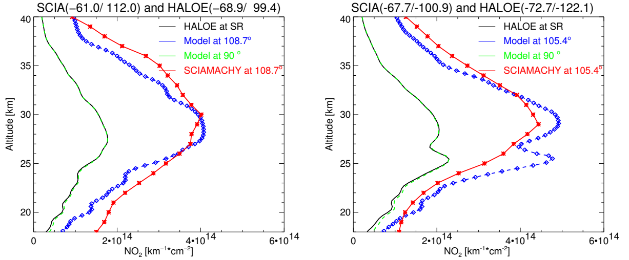
Figure 11. Examples of \text{NO}_2 profiles from SCIAMACHY lunar occultation version 2.2 compared with HALOE for 2003 (left) and 2004 (right). Red the SCIAMACHY result, blue the HALOE photochemically scaled to SCIAMACHY SZA, green the model result at HALOE SZA, and black the HALOE \text{NO}_2 profile.
